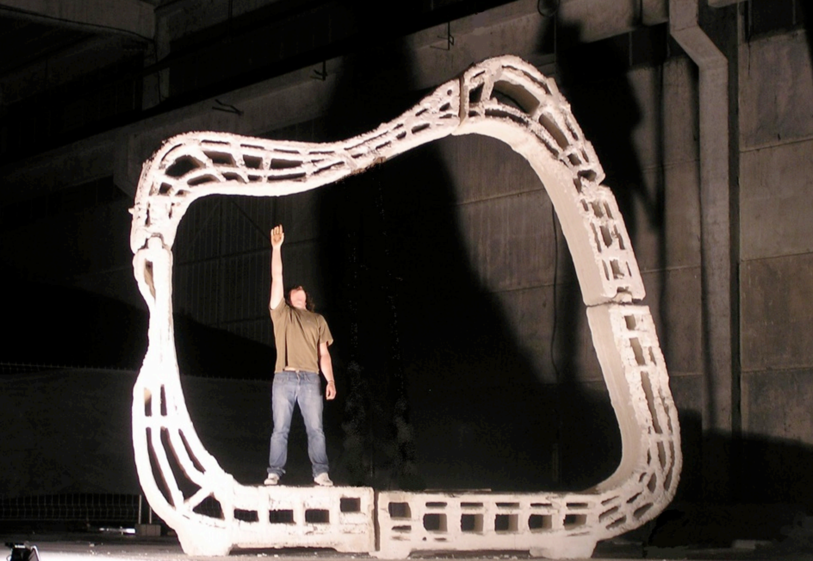
3D printed construction material – Roberto Dini
